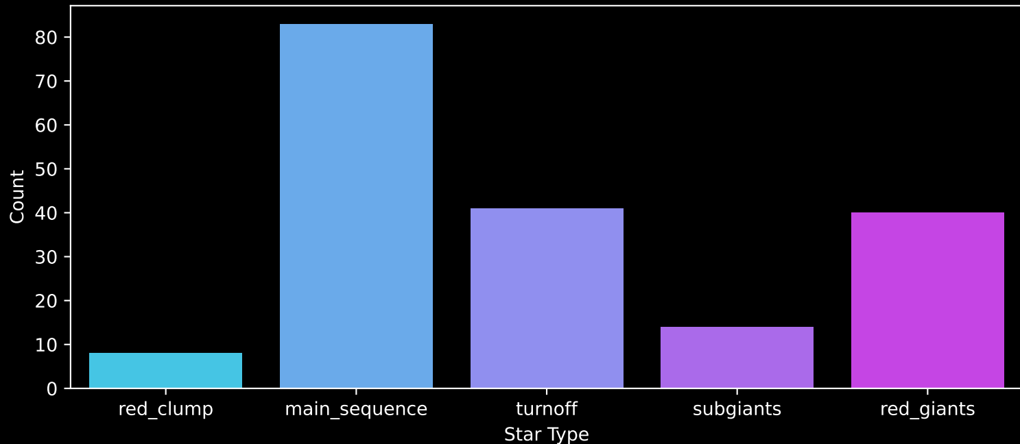
APOGEE DR17 Field: [281-39-O_TESS] Count plot of Star Type
