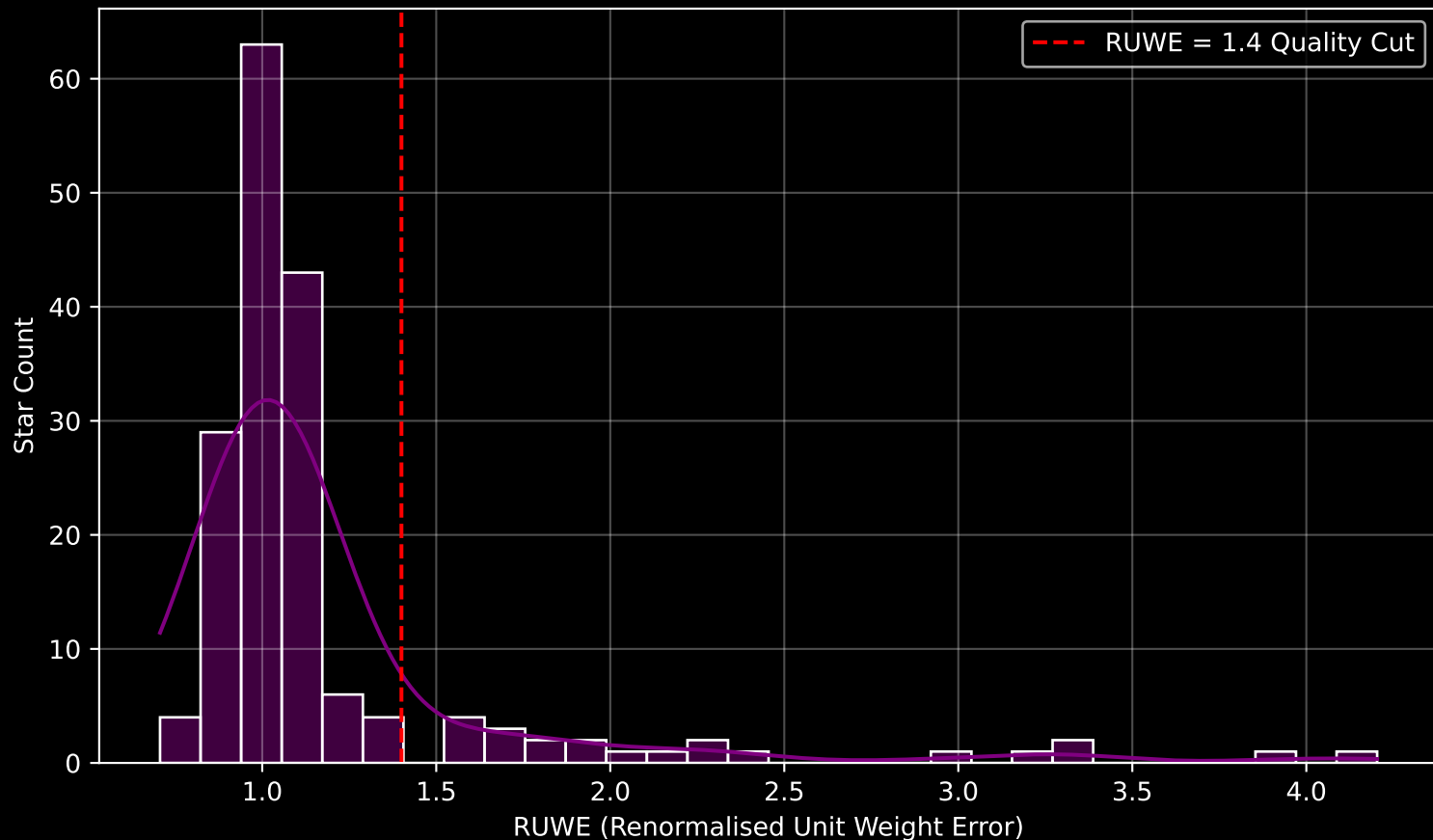
GAPOGEE DR17 Field [281-39-O_TESS] RUWE Distribution (n= 171)
