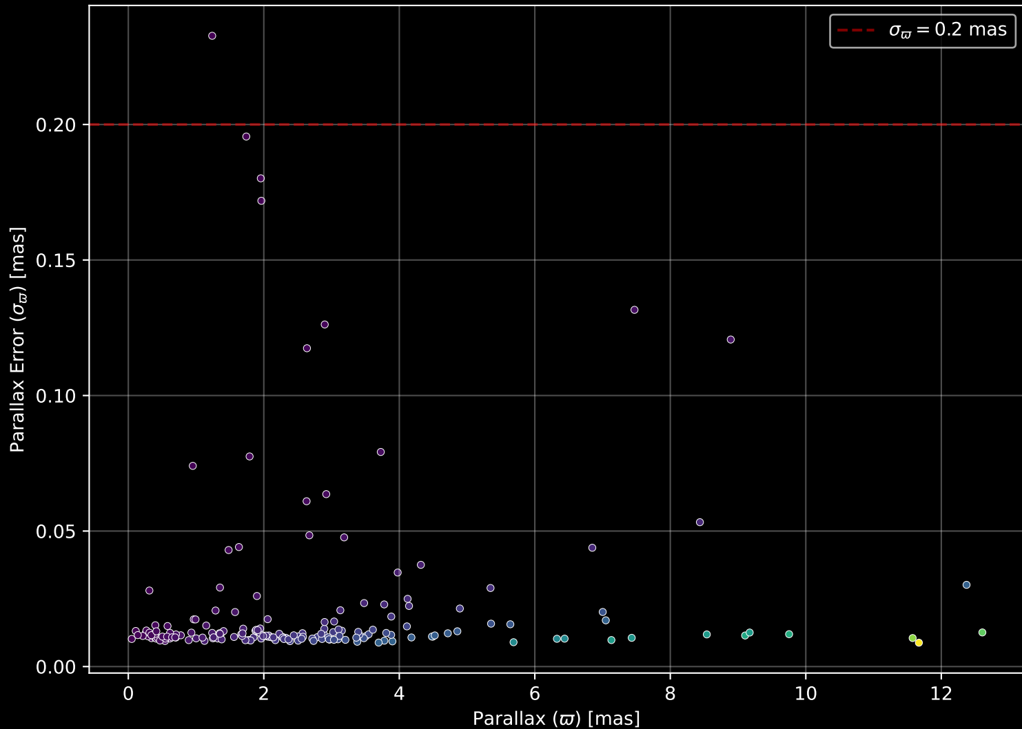
APOGEE DR17 Field: [281-39-O_TESS] Parallax Quality (n= 186)
